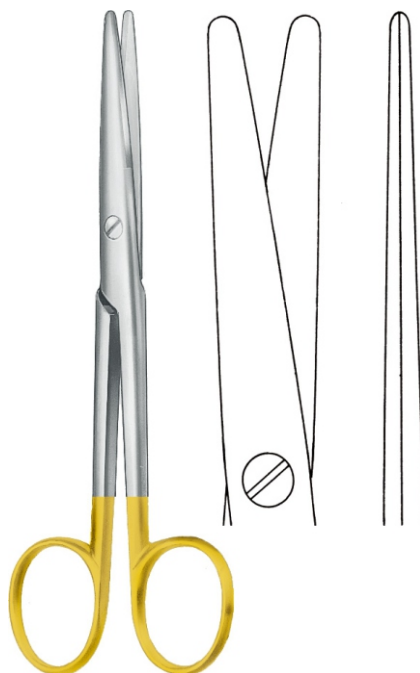
TC MAYO SCISSORS EV09164-14 beveled blades straight 5 1/2" (140mm) EV09164-17 beveled blades straight 6 1/4" (171mm) EV09164-23 beveled blades straight 9" (229mm)
